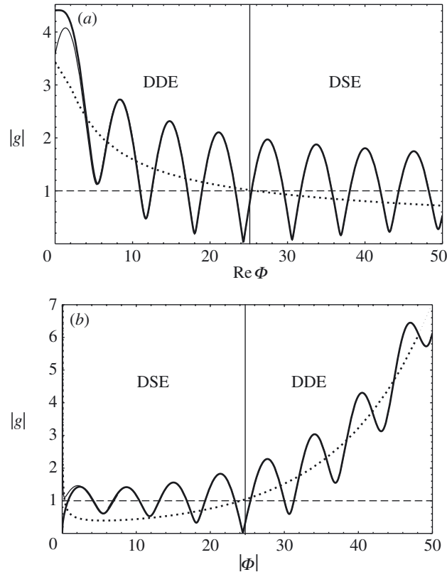
Figure 1. Modulus |g(\Phi)| , showing the transition between DSE and DDE for the Fresnel integral g_1(\Phi) (equation (3.4)) of § 3 a : (a) on a line with \text{Im } \Phi = 2.2 ; (b) on a ray with \arg \Phi = \pi/35 . Thick curves, exact |g| ; thin curves, the approximation (2.6); dashed lines, subdominant contribution (unity) to g ; dotted curves, dominant contribution to g (first term of (2.6)).
