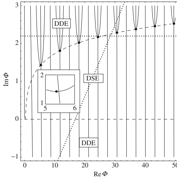
Figure 2. Contours of \arg(g(\Phi)) for the Fresnel integral g_1(\Phi) (equation (3.4)) of § 3 a at intervals of \pi/4 ; the contours cross at the zeros of g(\Phi) . Filled circles, approximate zeros calculated from (2.6); dashed curves, the boundary between the regions of DSE and DDE, calculated from (2.8); dotted lines, lines along which the graphs of |g| in figure 1 were calculated. The inset is a magnification near the smallest zero, illustrating the high accuracy of the approximation based on (2.6).
