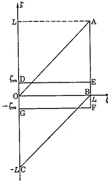
FIGURE 4. Domain of integration of (13).
