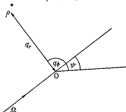
FIGURE 2. Coordinates in the q_r, q_\phi plane in \rho^* space.
