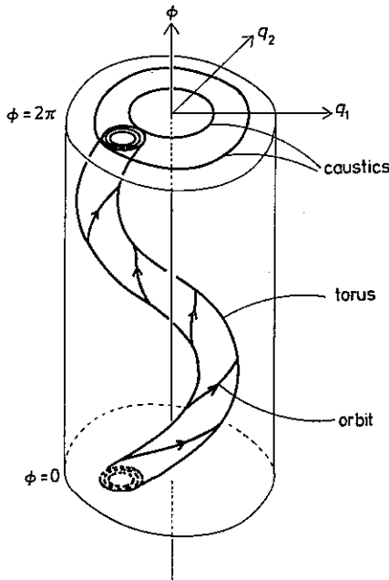
Figure 2. Energy 'surface' \mathcal{S} with coordinates (q_1, q_2, \phi) ( \phi = 0 and \phi = 2\pi are identified). The torus corresponding to an orbit with constant angular momentum is shown, and the caustics which envelop its projection along \phi .
