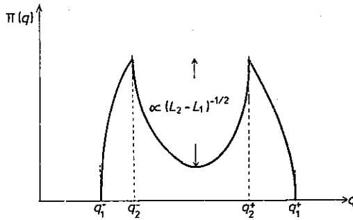
Figure 4. Local average probability density arising from projection of phase space region with constant energy between two tori corresponding to motions with angular momenta L_1 and L_2 .
