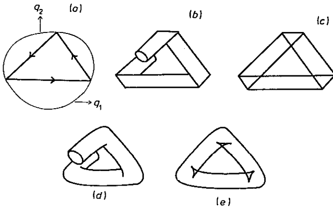
Figure 3. (a) Stable isolated closed orbit on billiard table; (b) torus in q_1, q_2, \phi space ( \phi perpendicular to paper) inhabited by nearby quasi-periodic orbit; (c) caustic resulting from projection of (b); (d) generification of torus in (b) resulting from softening potential at the boundary; (e) caustic resulting from projection of (d).
