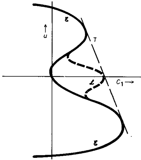
Figure 4. The classical manifold \mathcal{Z} and catastrophe line \mathcal{L} (broken curve) of a swallowtail Wigner catastrophe, for C_2 > 0 , C_3 < 0 . 'T' is the common tangent with equation C_1 = \frac{1}{4}C_3^2 - C_2u .
