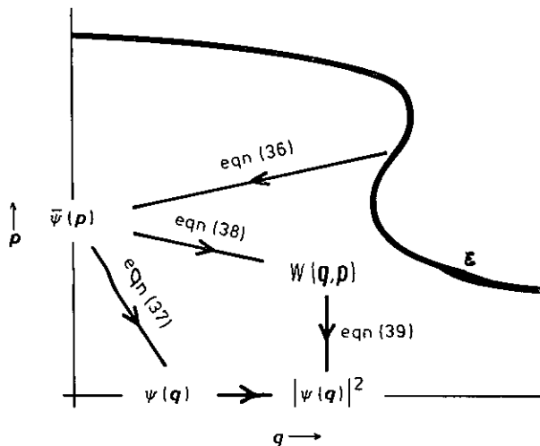
Figure 1. Manifold \mathcal{E} of classical trajectories, leading to formulae for the coordinate and momentum wavefunctions and the Wigner function.
