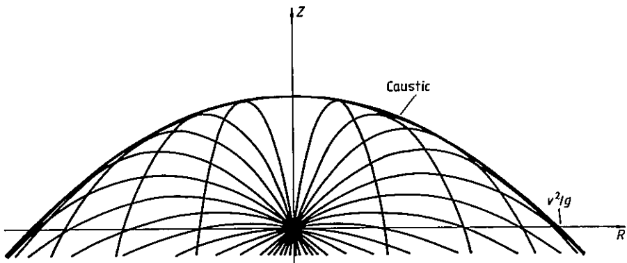
Figure 1. 'Gravity's rainbow' enveloping the orbits of falling particles emitted by a source.
