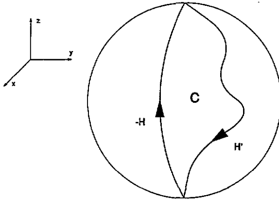
Figure 1. The cycle C on the sphere \|\mathbf{B}\| = B is composed of the two half-cycles H' and -H .
